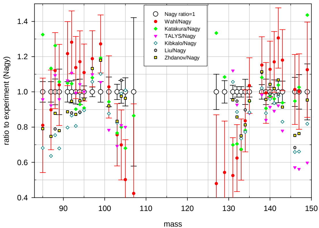
Benchmark A: ^{238}\text{U} at 5.5 MeV, post neutron emission yield ratios to Nagy's experimental data lower graph: partial plot (very low and high values omitted)
